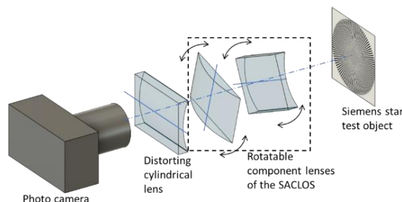
Fig. 1. Schematic diagram of the optical system used in the experiments.
