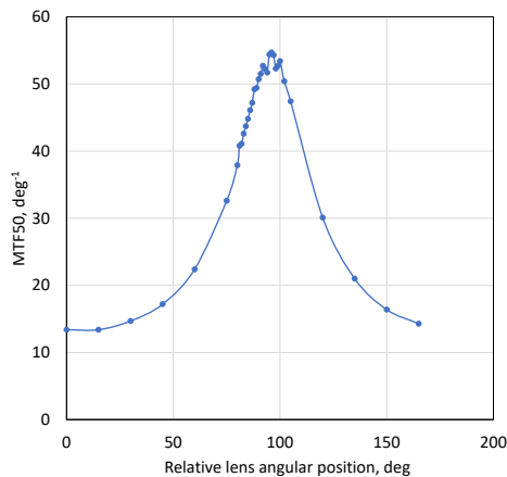
Fig. 3. A plot of the MTF50 dependence on the position angle of one element of the SACLOS, with the other element's angle being fixed.
